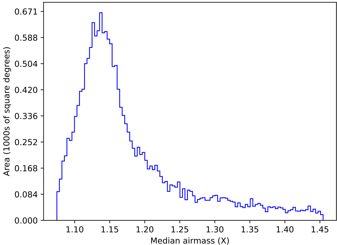
too_elab_r8_d3_gz_v3.4_10yrs WFD u band: Median airmass
