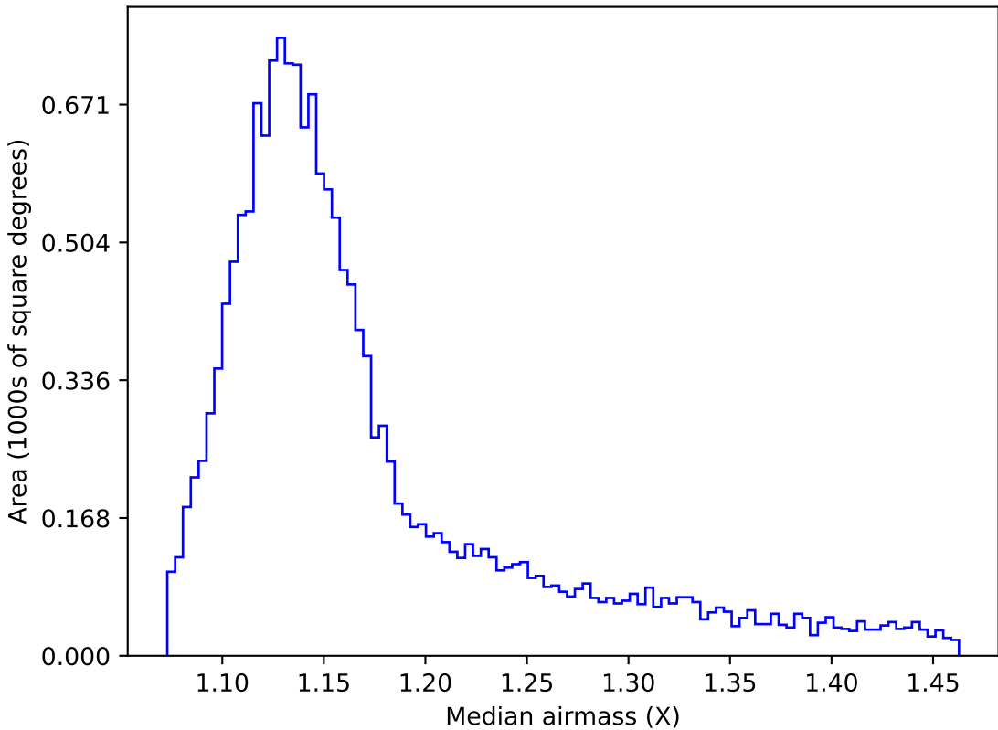
too_elab_r8_d3_gz_v3.4_10yrs WFD r band: Median airmass
