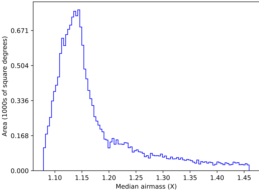
too_elab_r8_d3_gz_v3.4_10yrs WFD i band: Median airmass
