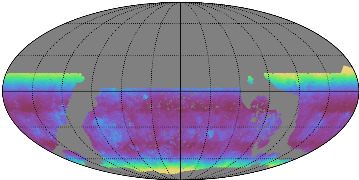
too_elab_r8_d3_gz_v3.4_10yrs WFD g band: Median airmass
