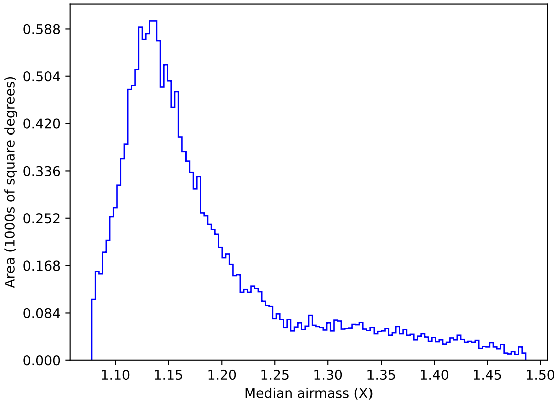
too_elab_r8_d3_gz_v3.4_10yrs WFD g band: Median airmass
