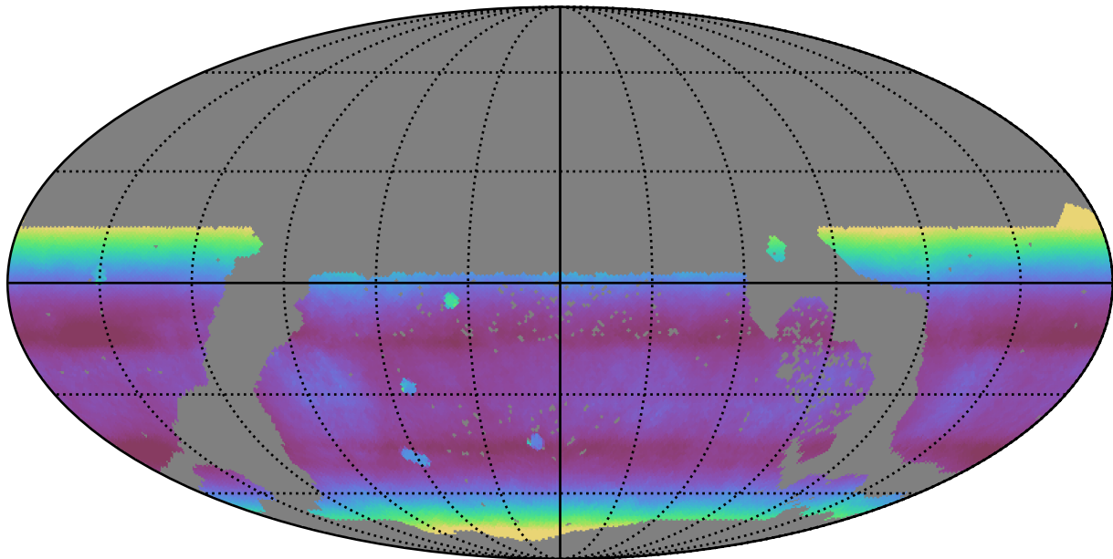
too_elab_r8_d3_gz_v3.4_10yrs WFD all bands: Median airmass
