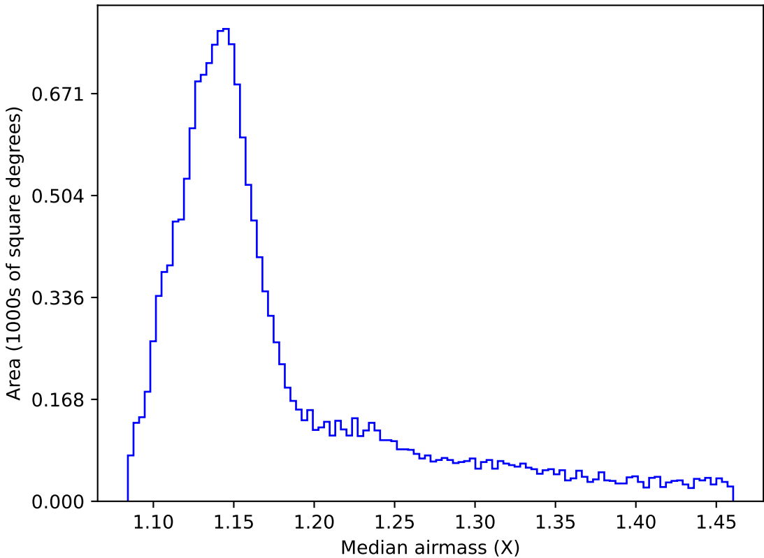
too_elab_r8_d3_gz_v3.4_10yrs WFD all bands: Median airmass
