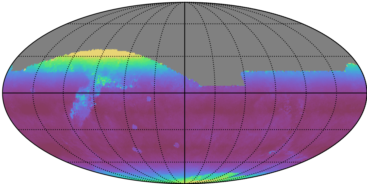
too_elab_r8_d3_gz_v3.4_10yrs All sky z band: Median airmass
