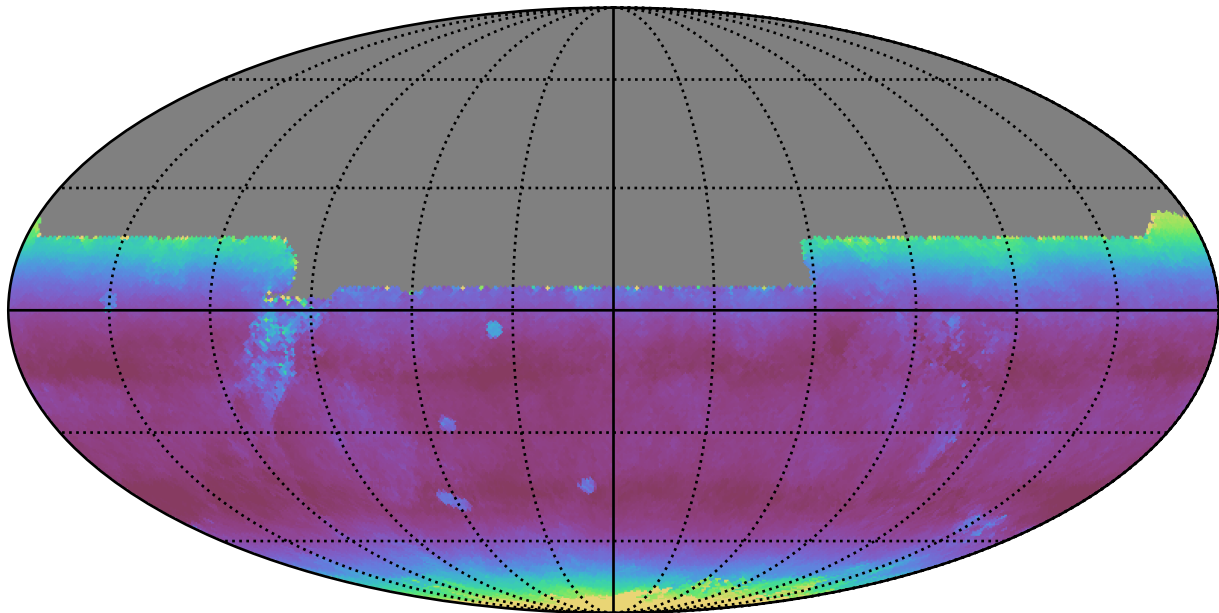
too_elab_r8_d3_gz_v3.4_10yrs All sky y band: Median airmass
