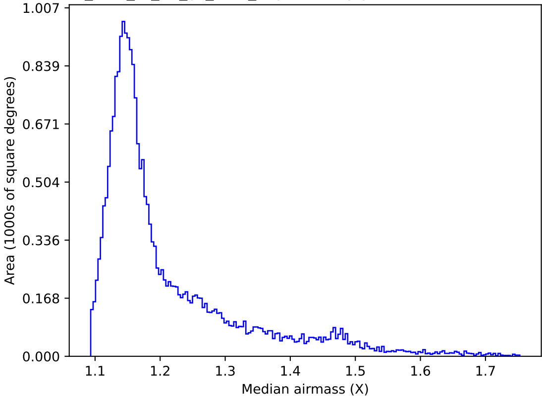
too_elab_r8_d3_gz_v3.4_10yrs All sky y band: Median airmass
