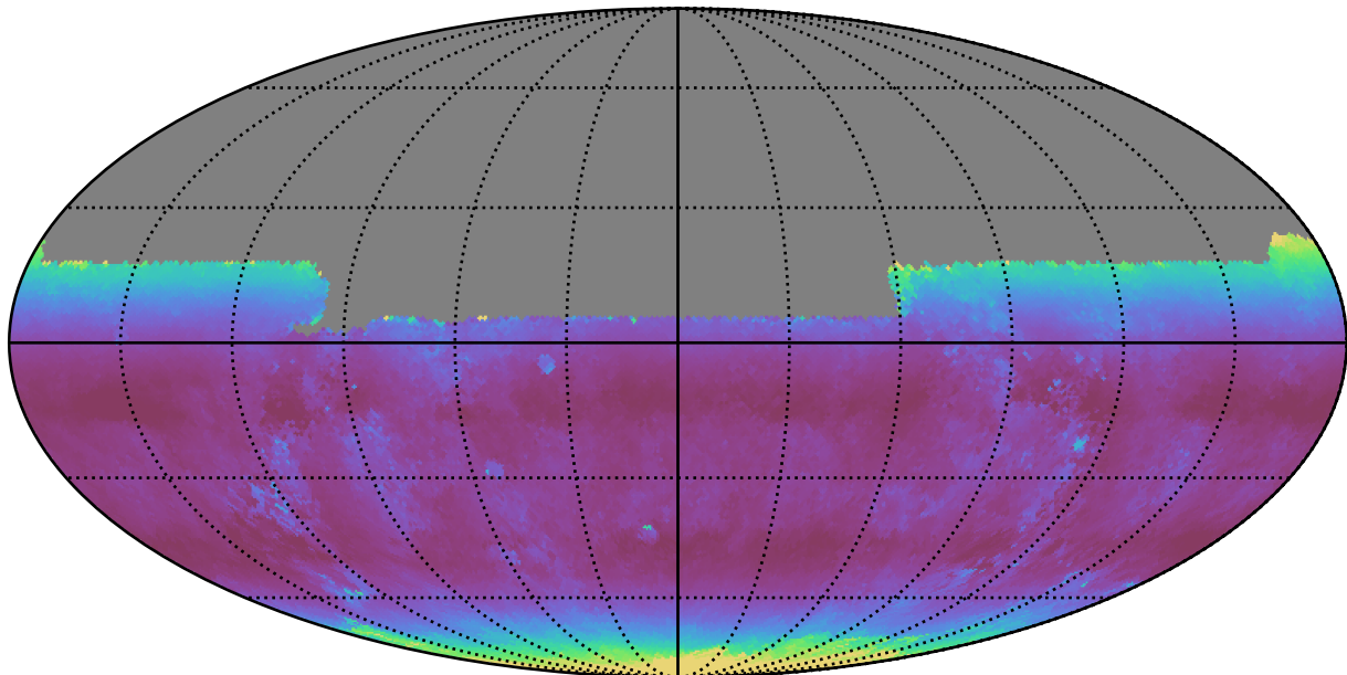
too_elab_r8_d3_gz_v3.4_10yrs All sky u band: Median airmass
