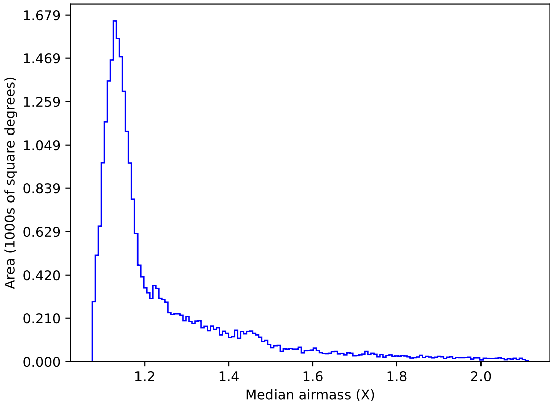
too_elab_r8_d3_gz_v3.4_10yrs All sky r band: Median airmass
