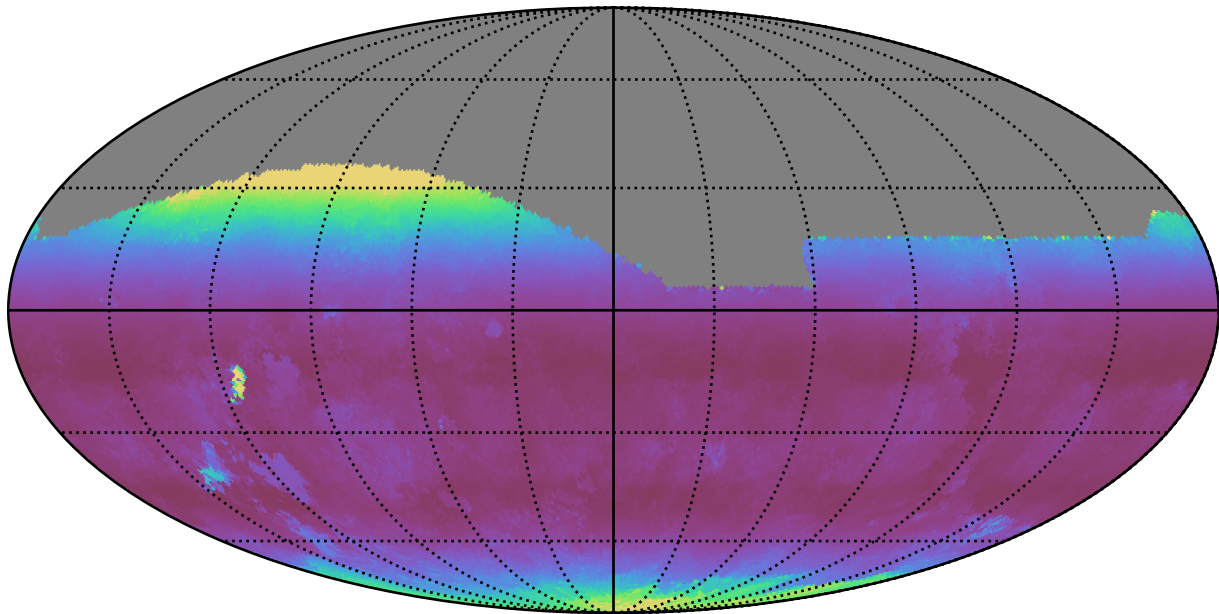
too_elab_r8_d3_gz_v3.4_10yrs All sky g band: Median airmass
