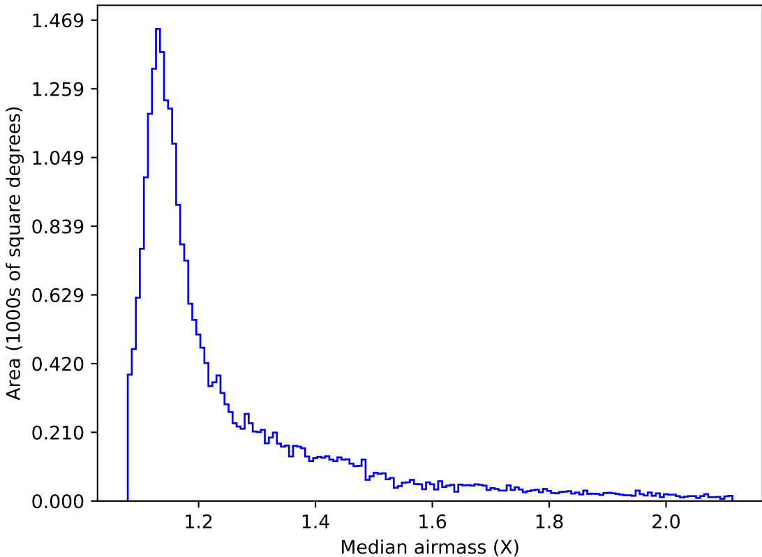
too_elab_r8_d3_gz_v3.4_10yrs All sky g band: Median airmass
