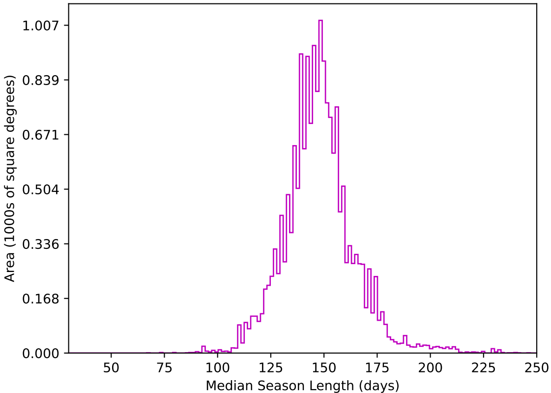
too_elab_r8_d3_gz_v3.4_10yrs WFD z band: Median Season Length
