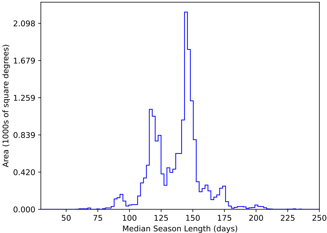
too_elab_r8_d3_gz_v3.4_10yrs WFD y band: Median Season Length
