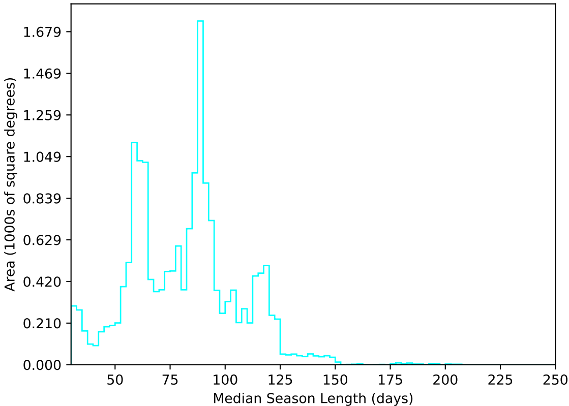
too_elab_r8_d3_gz_v3.4_10yrs WFD u band: Median Season Length
