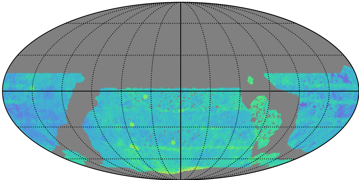
too_elab_r8_d3_gz_v3.4_10yrs WFD i band: Median Season Length
