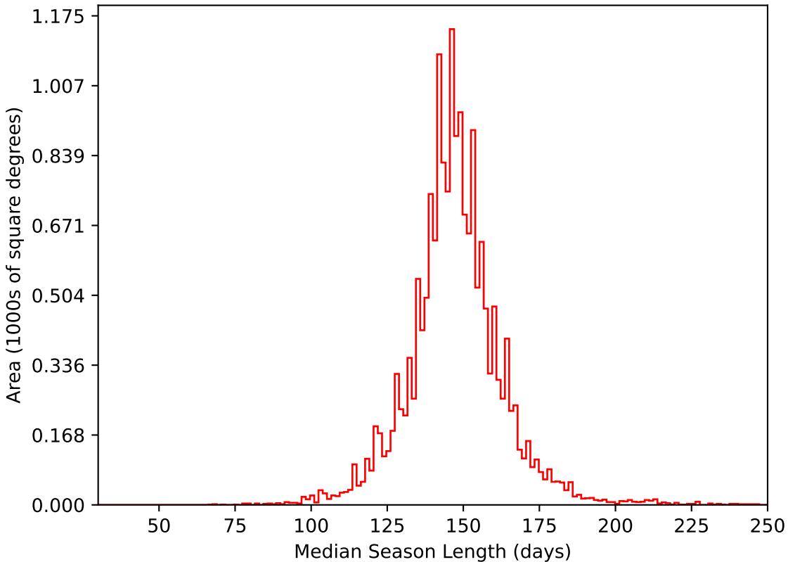
too_elab_r8_d3_gz_v3.4_10yrs WFD i band: Median Season Length
