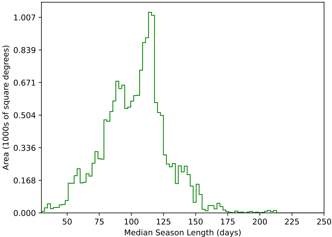
too_elab_r8_d3_gz_v3.4_10yrs WFD g band: Median Season Length
