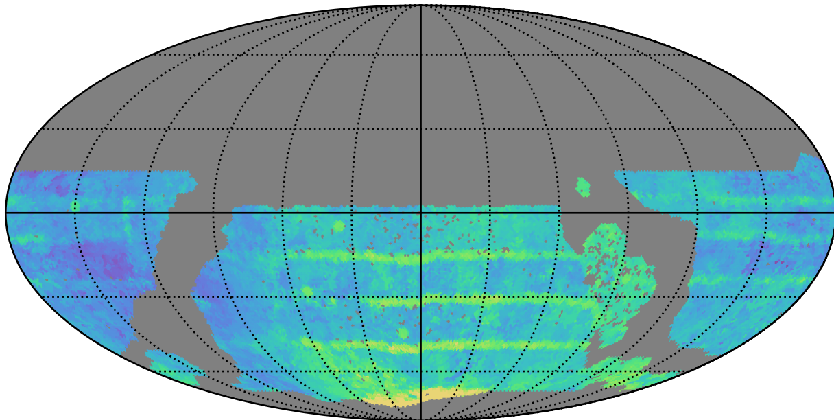
too_elab_r8_d3_gz_v3.4_10yrs WFD all bands: Median Season Length
