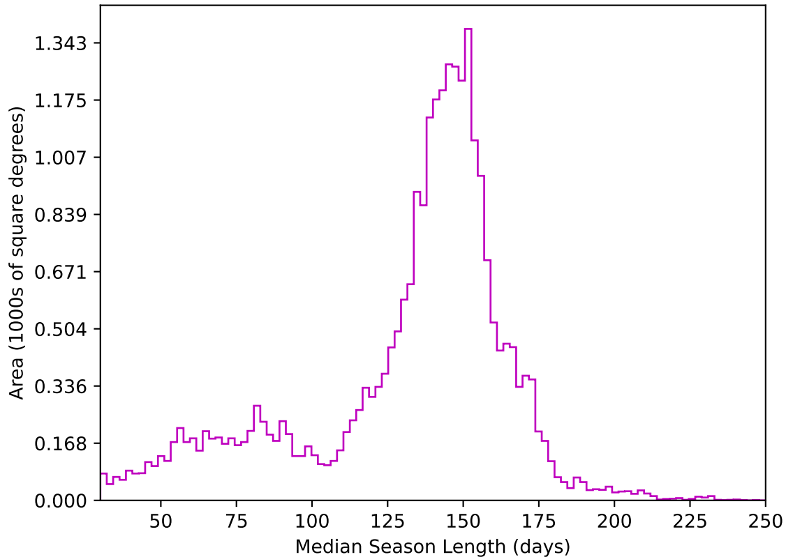
too_elab_r8_d3_gz_v3.4_10yrs All sky z band: Median Season Length
