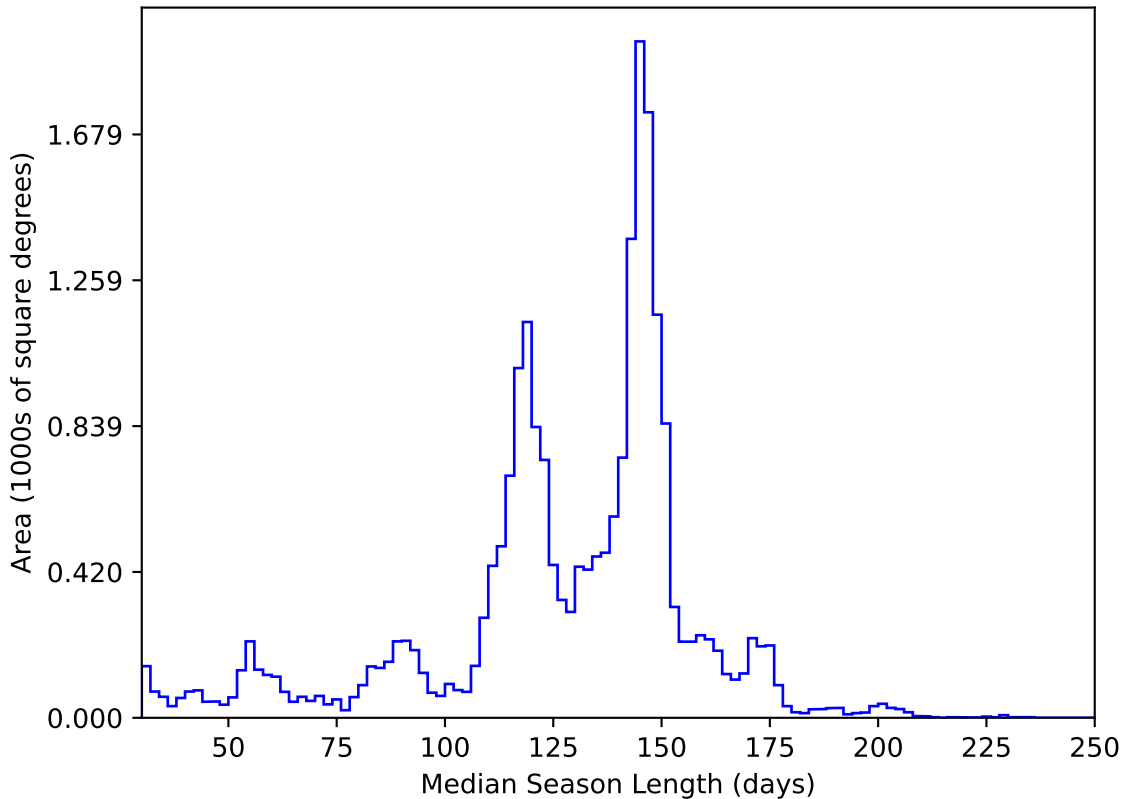
too_elab_r8_d3_gz_v3.4_10yrs All sky y band: Median Season Length
