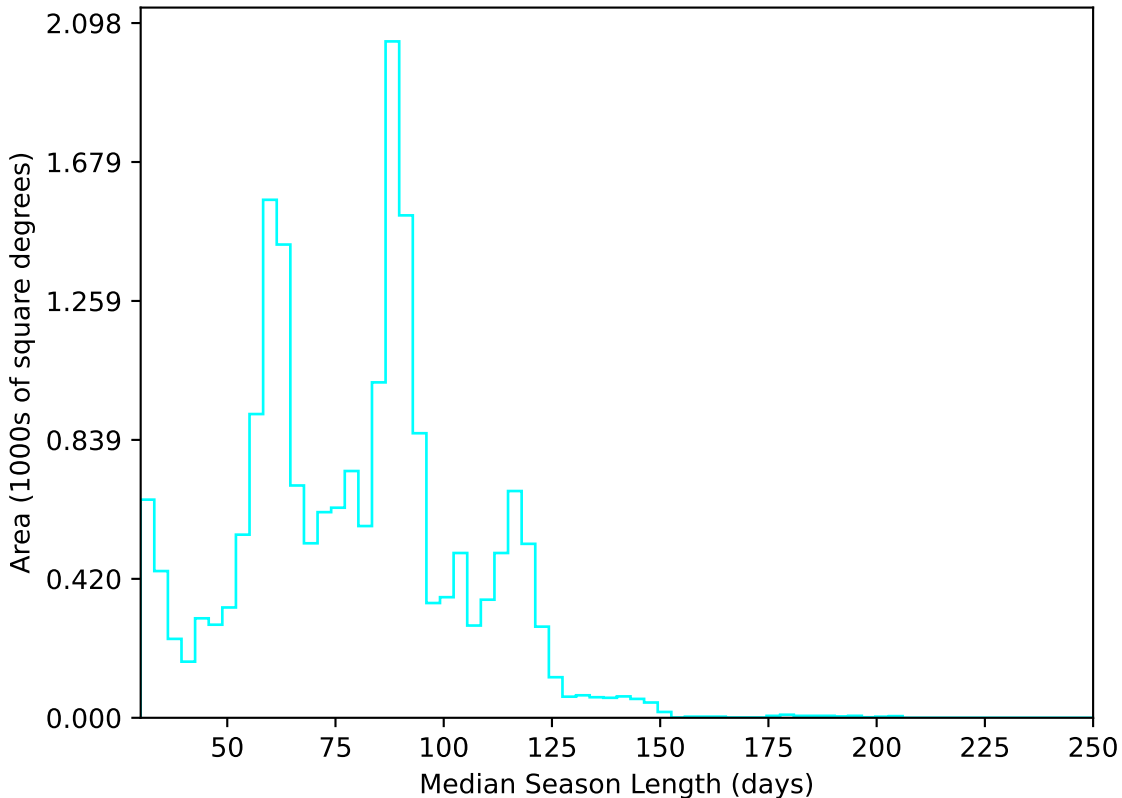
too_elab_r8_d3_gz_v3.4_10yrs All sky u band: Median Season Length
