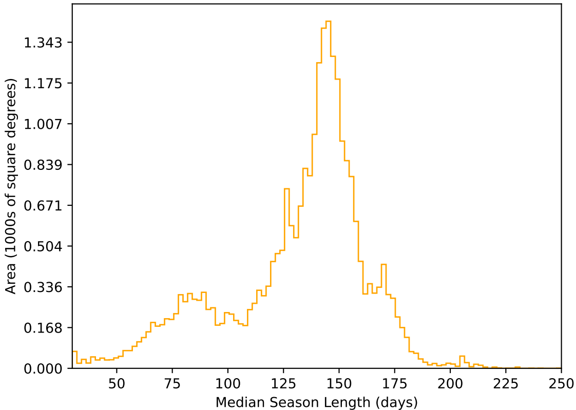
too_elab_r8_d3_gz_v3.4_10yrs All sky r band: Median Season Length
