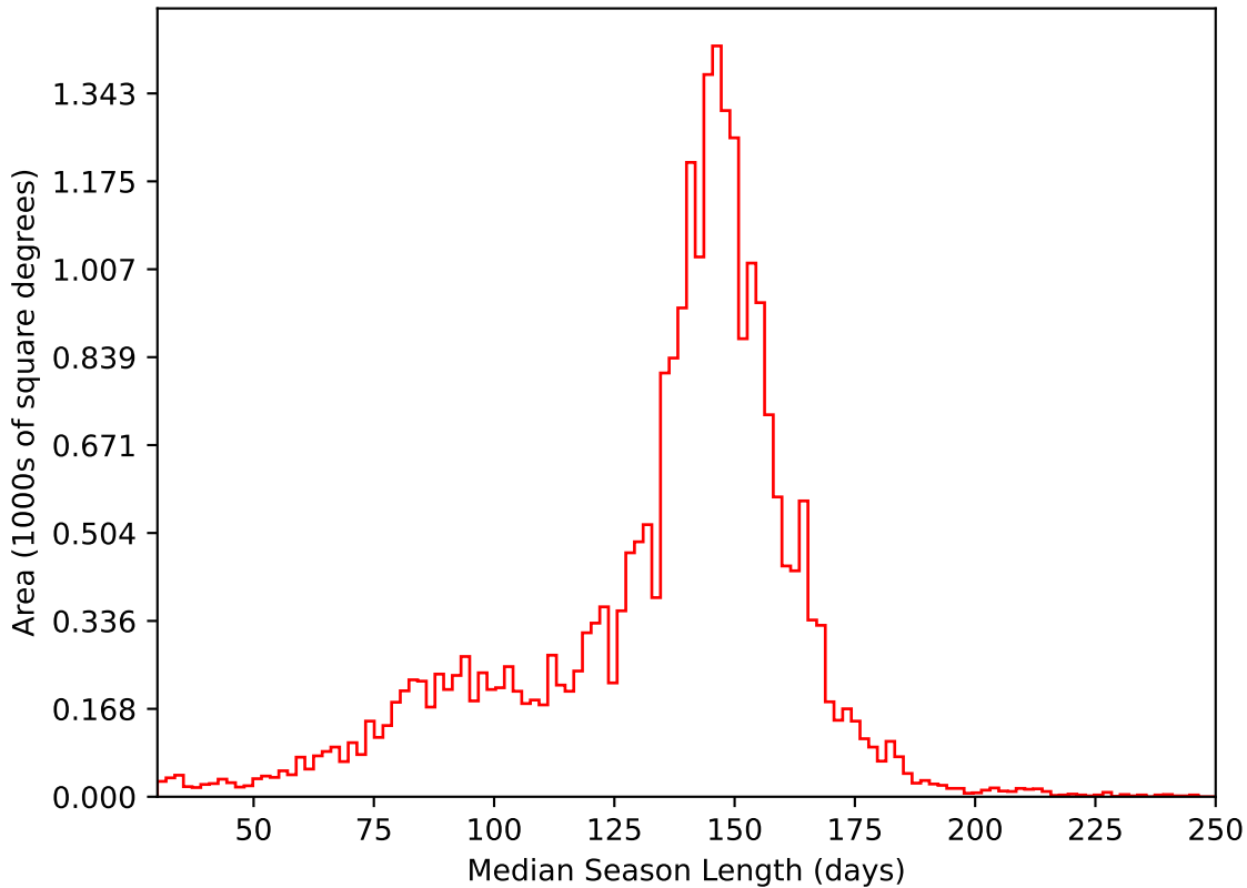
too_elab_r8_d3_gz_v3.4_10yrs All sky i band: Median Season Length
