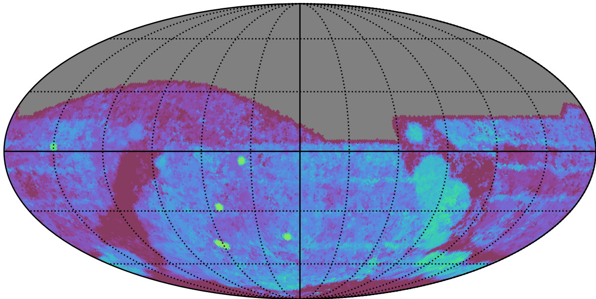
too_elab_r8_d3_gz_v3.4_10yrs All sky g band: Median Season Length
