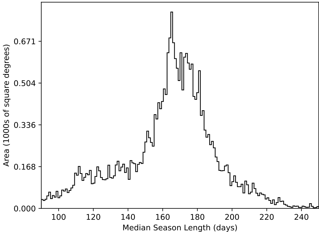
too_elab_r8_d3_gz_v3.4_10yrs All sky all bands: Median Season Length
