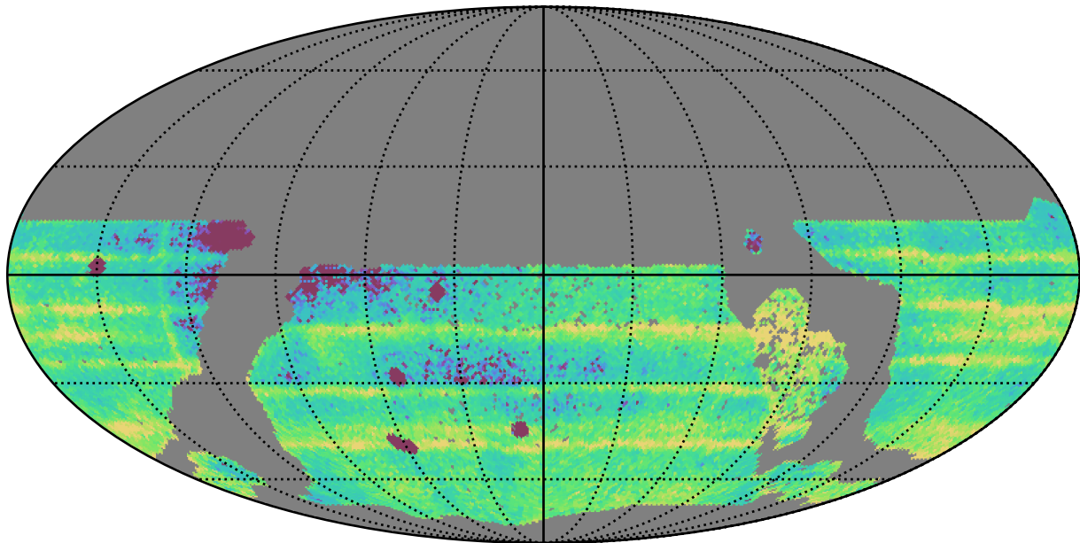
too_elab_r8_d3_gz_v3.4_10yrs WFD: Median Intra-Night Gap
