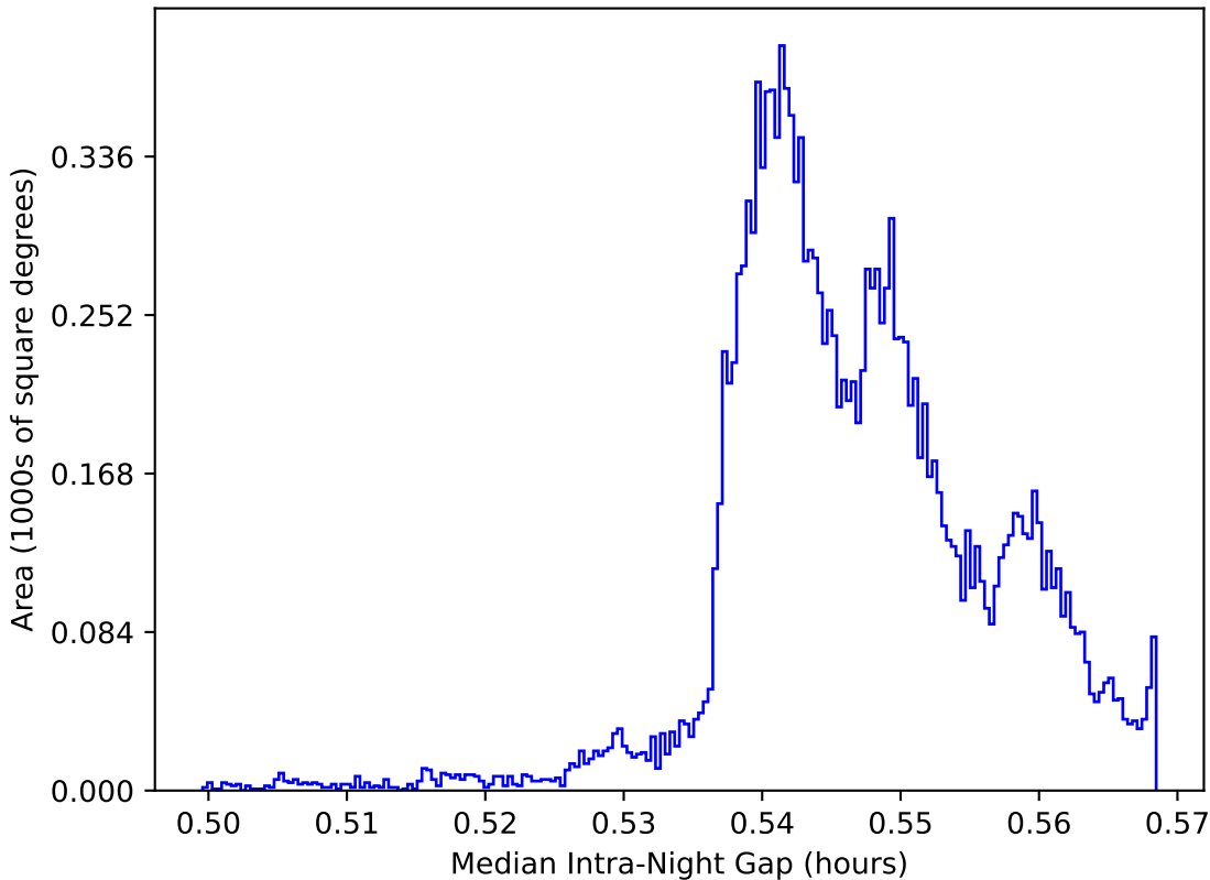
too_elab_r8_d3_gz_v3.4_10yrs WFD: Median Intra-Night Gap
