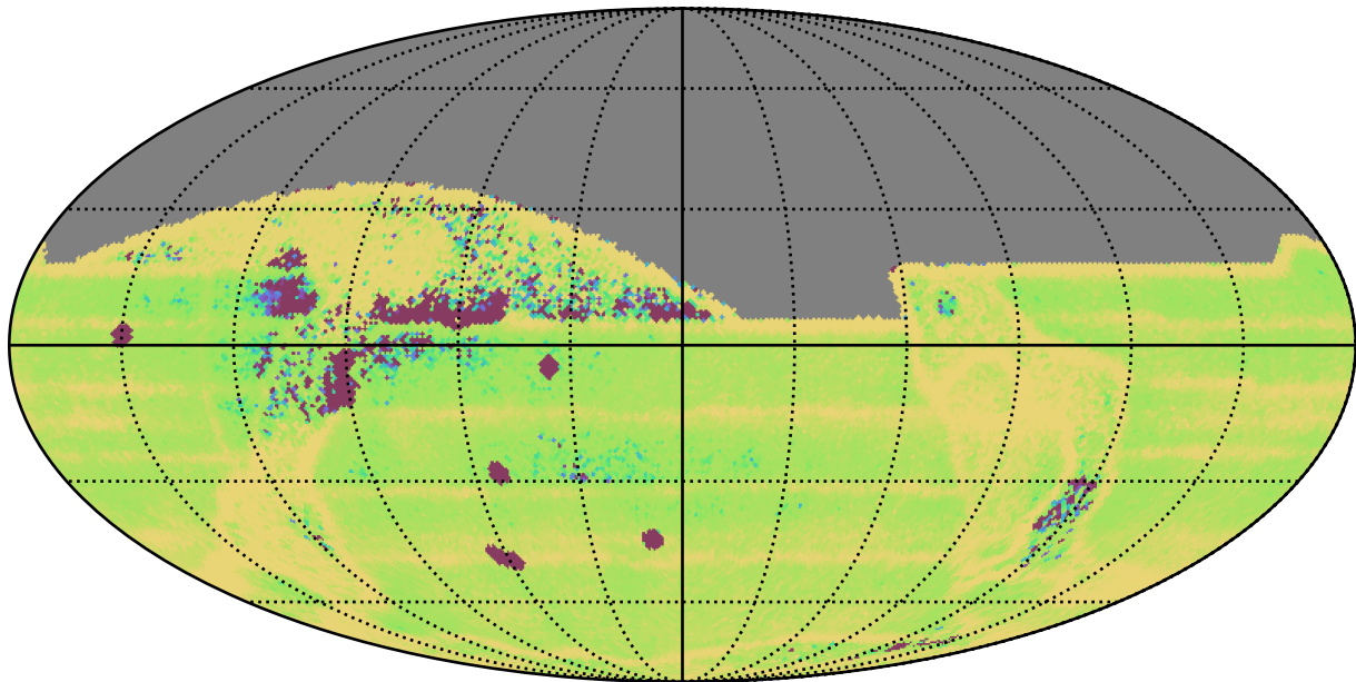
too_elab_r8_d3_gz_v3.4_10yrs All sky: Median Intra-Night Gap
