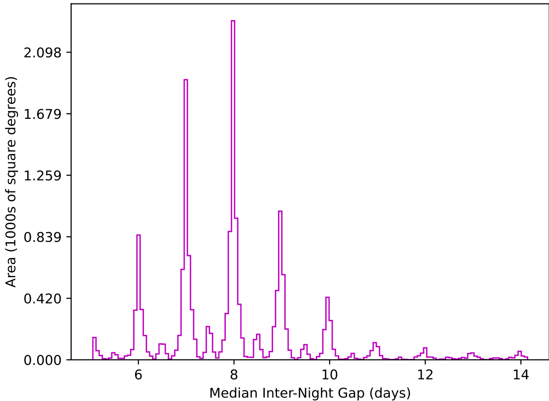
too_elab_r8_d3_gz_v3.4_10yrs WFD z band: Median Inter-Night Gap
