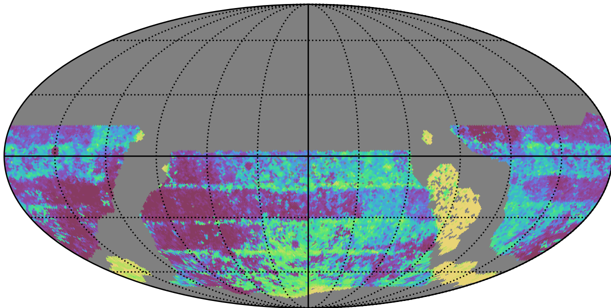
too_elab_r8_d3_gz_v3.4_10yrs WFD y band: Median Inter-Night Gap
