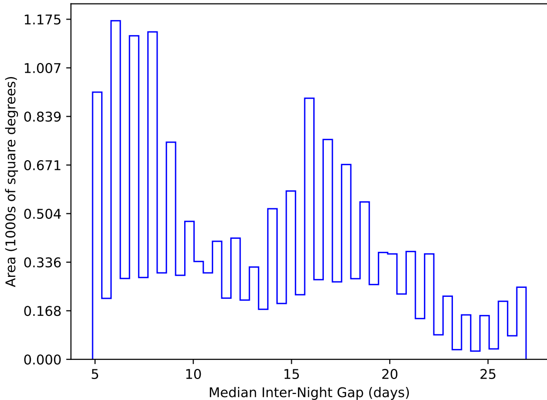
too_elab_r8_d3_gz_v3.4_10yrs WFD y band: Median Inter-Night Gap
