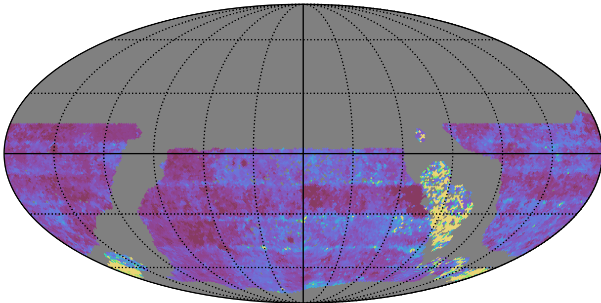
too_elab_r8_d3_gz_v3.4_10yrs WFD u band: Median Inter-Night Gap
