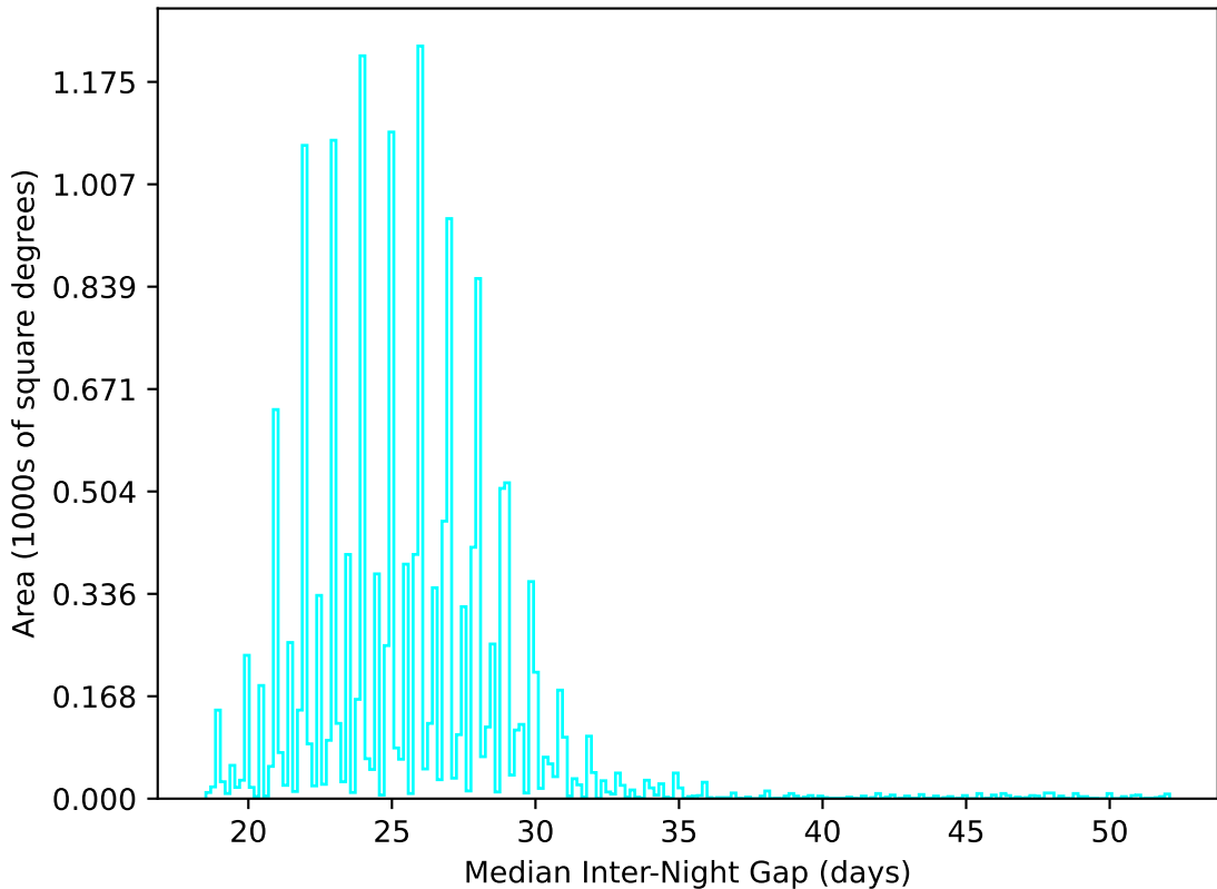
too_elab_r8_d3_gz_v3.4_10yrs WFD u band: Median Inter-Night Gap
