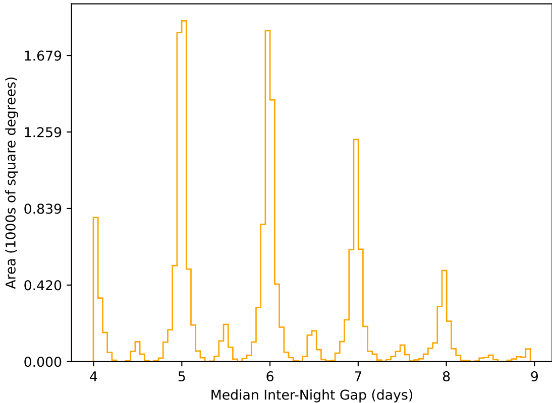
too_elab_r8_d3_gz_v3.4_10yrs WFD r band: Median Inter-Night Gap
