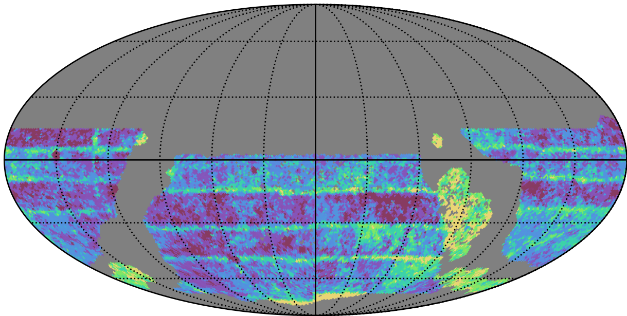
too_elab_r8_d3_gz_v3.4_10yrs WFD i band: Median Inter-Night Gap
