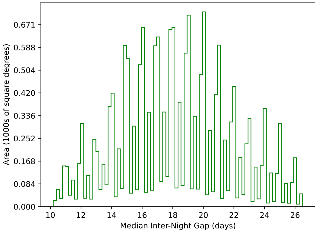
too_elab_r8_d3_gz_v3.4_10yrs WFD g band: Median Inter-Night Gap
