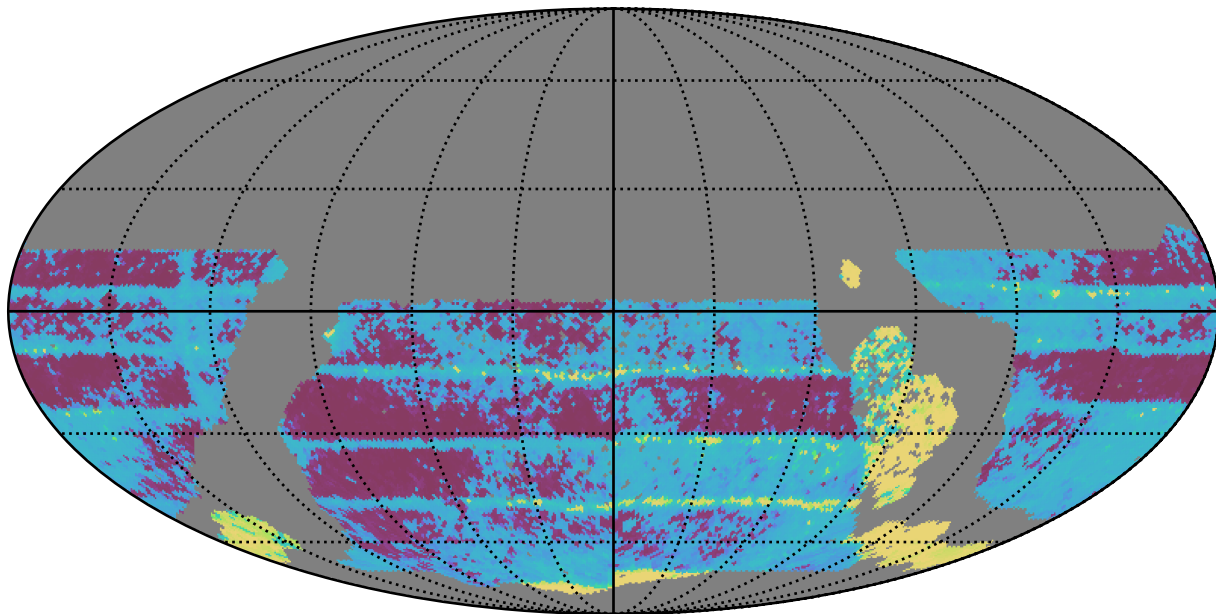
too_elab_r8_d3_gz_v3.4_10yrs WFD all bands: Median Inter-Night Gap
