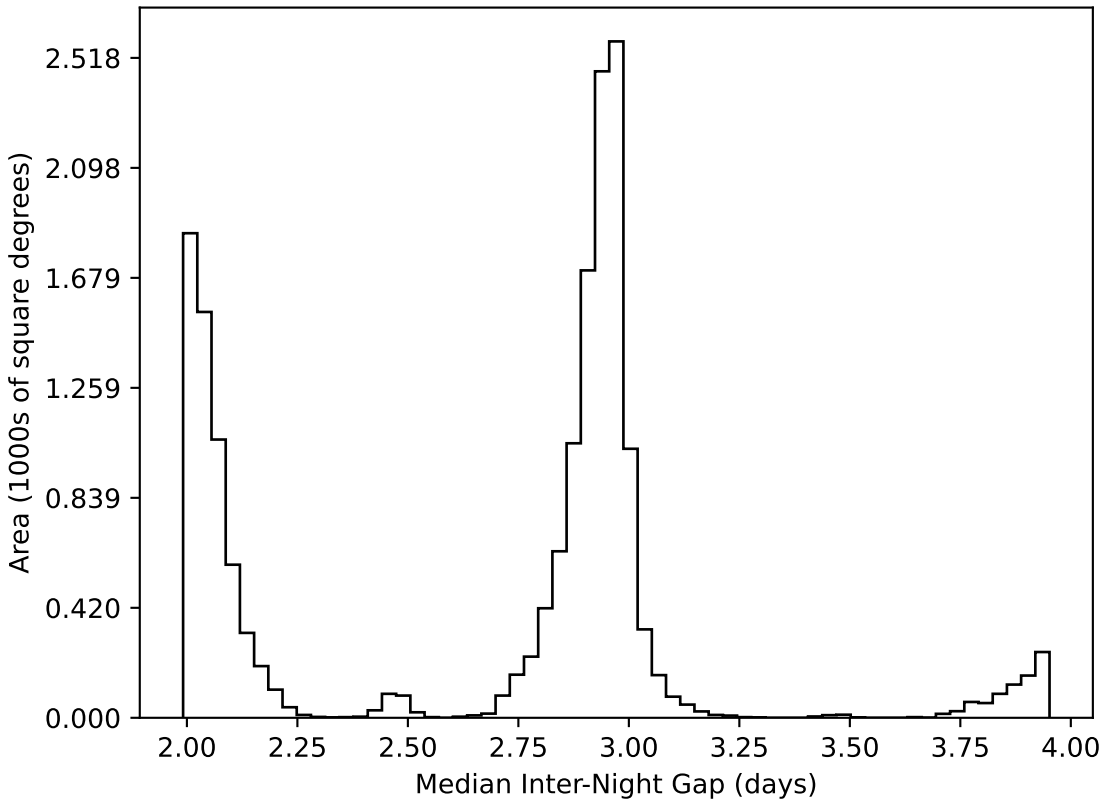
too_elab_r8_d3_gz_v3.4_10yrs WFD all bands: Median Inter-Night Gap
