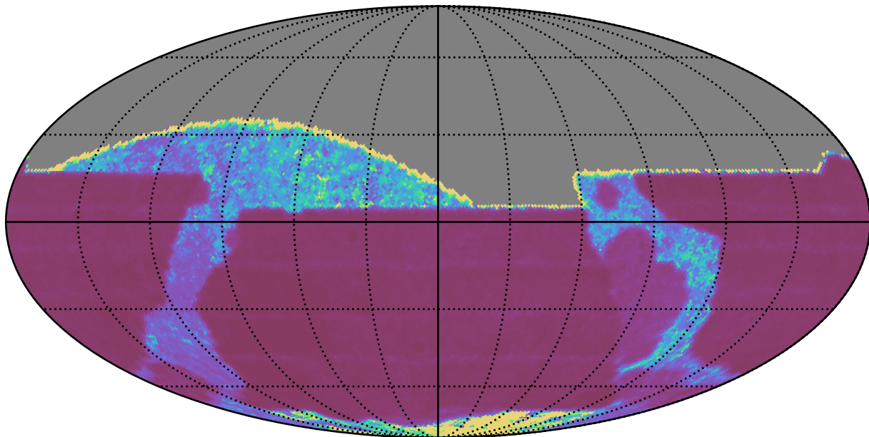
too_elab_r8_d3_gz_v3.4_10yrs All sky z band: Median Inter-Night Gap
