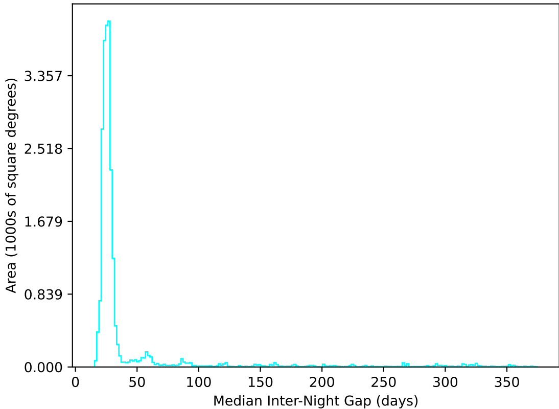
too_elab_r8_d3_gz_v3.4_10yrs All sky u band: Median Inter-Night Gap
