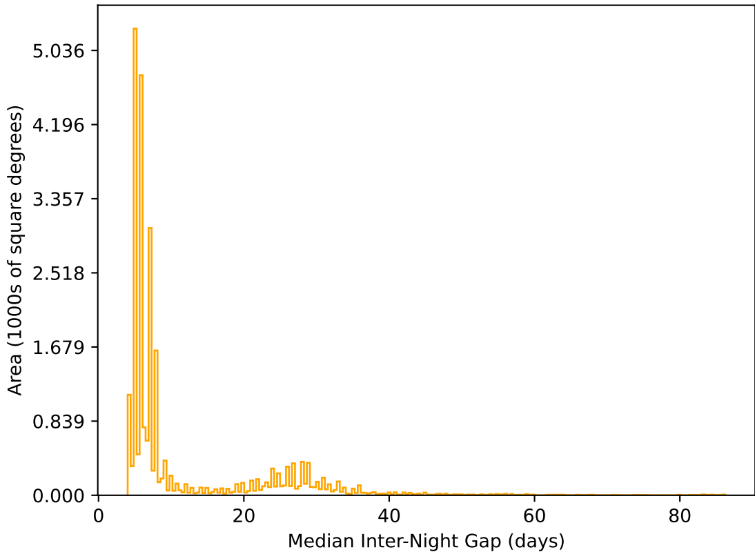
too_elab_r8_d3_gz_v3.4_10yrs All sky r band: Median Inter-Night Gap
