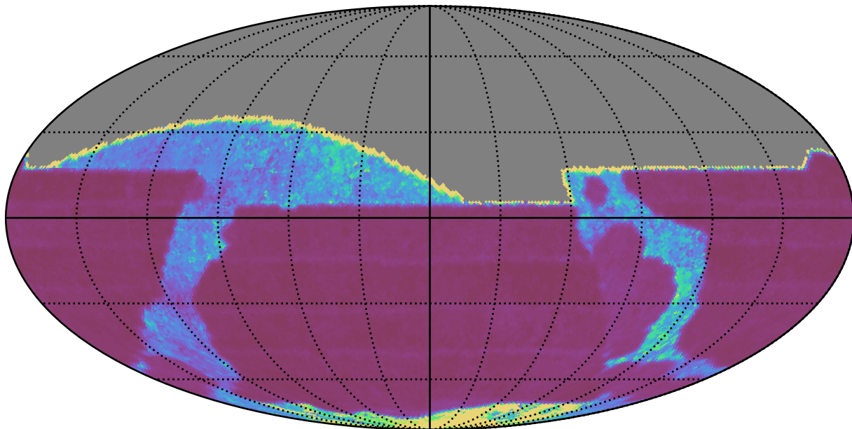
too_elab_r8_d3_gz_v3.4_10yrs All sky i band: Median Inter-Night Gap
