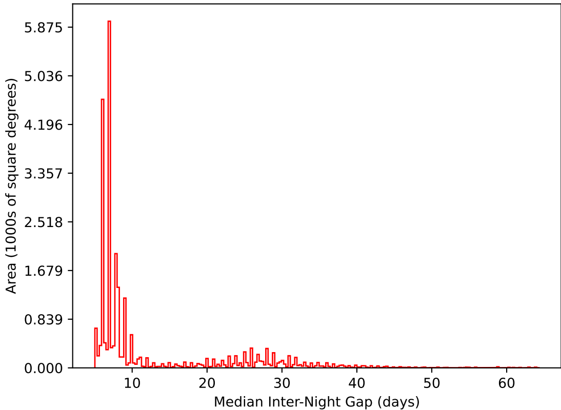
too_elab_r8_d3_gz_v3.4_10yrs All sky i band: Median Inter-Night Gap
