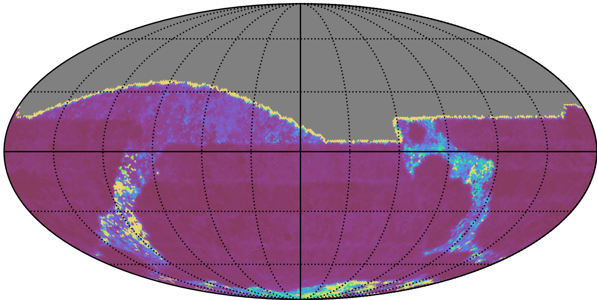
too_elab_r8_d3_gz_v3.4_10yrs All sky g band: Median Inter-Night Gap
