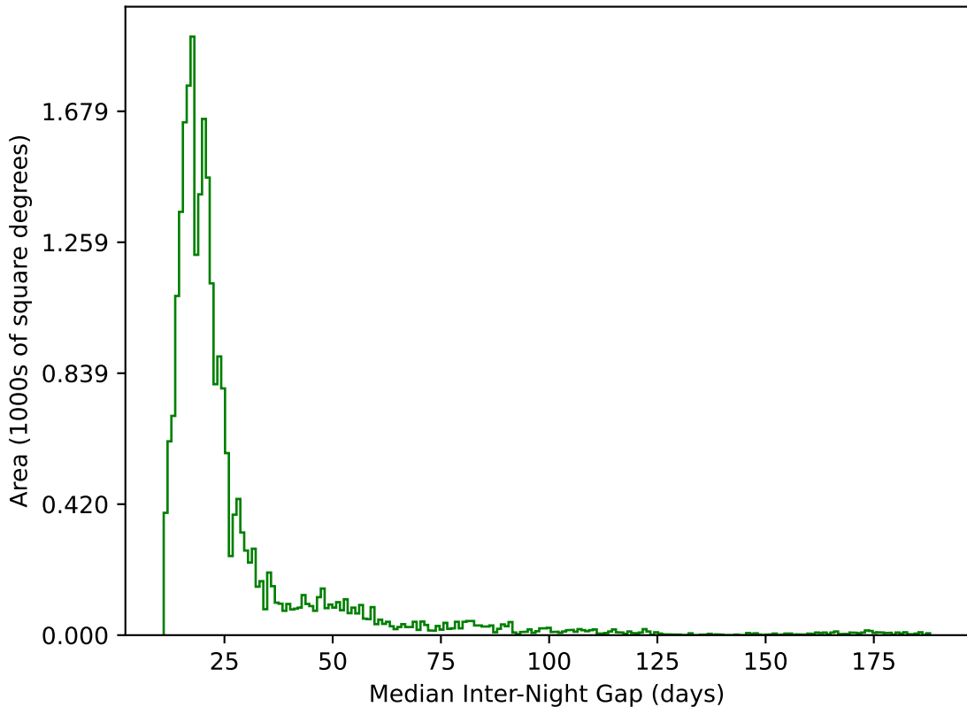
too_elab_r8_d3_gz_v3.4_10yrs All sky g band: Median Inter-Night Gap
