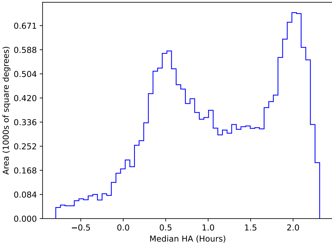
too_elab_r8_d3_gz_v3.4_10yrs WFD z band: Median HA
