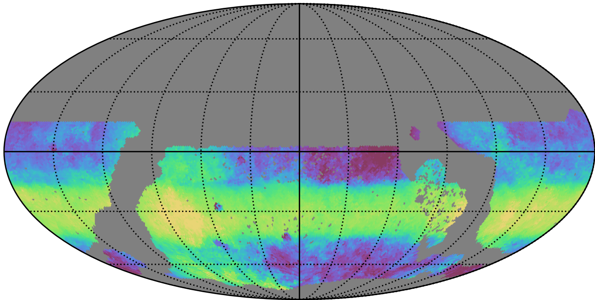
too_elab_r8_d3_gz_v3.4_10yrs WFD y band: Median HA
